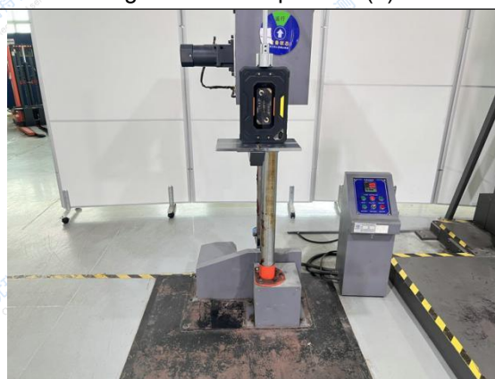
Fig.59 Test setup- Face (6)
