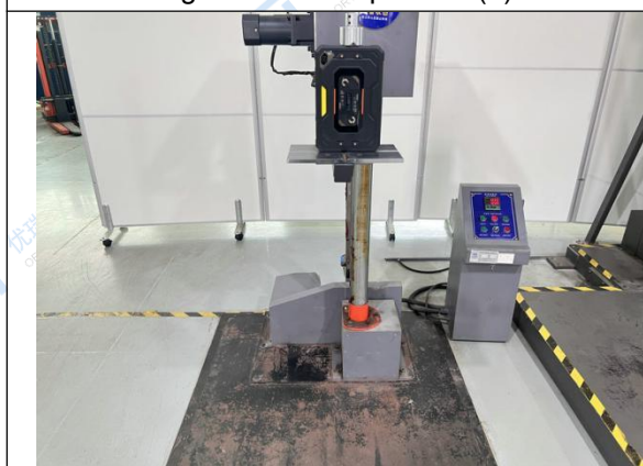
Fig.58 Test setup- Face (5)
