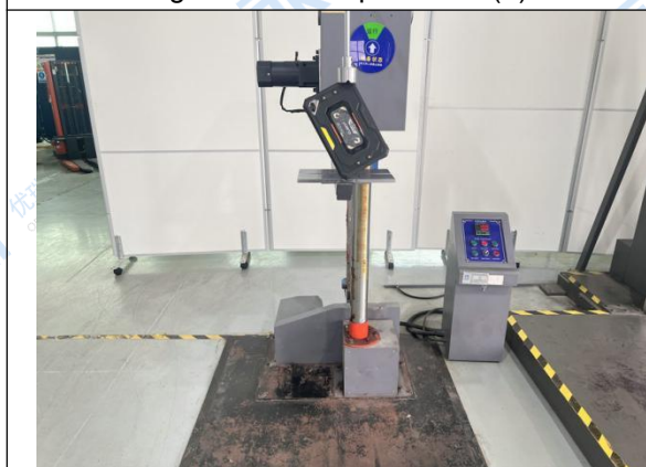
Fig.62 Test setup- Corner (3)
