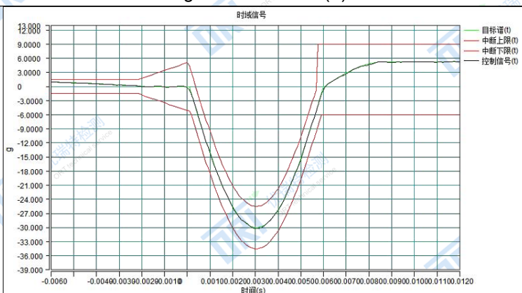
Fig.92 Test Curve (-)
