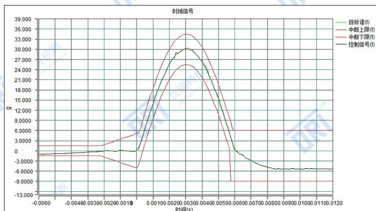
Fig.91 Test Curve (+)
