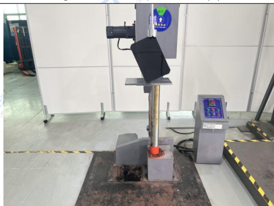
Fig.66 Test setup- Corner (7)
