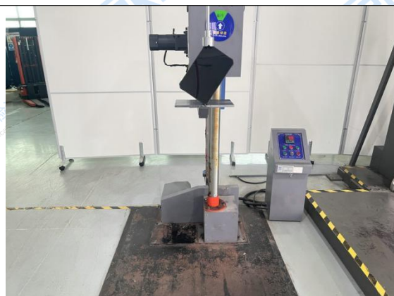
Fig.65 Test setup- Corner (6)
