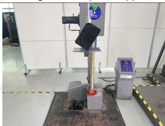
Fig.63 Test setup- Corner (4)
