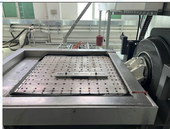
Fig.43 Test setup (Y axis)
