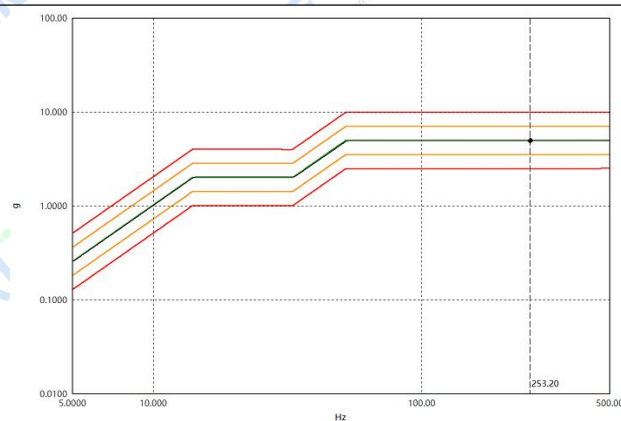
Fig.45 Test Spectrum (X axis)
