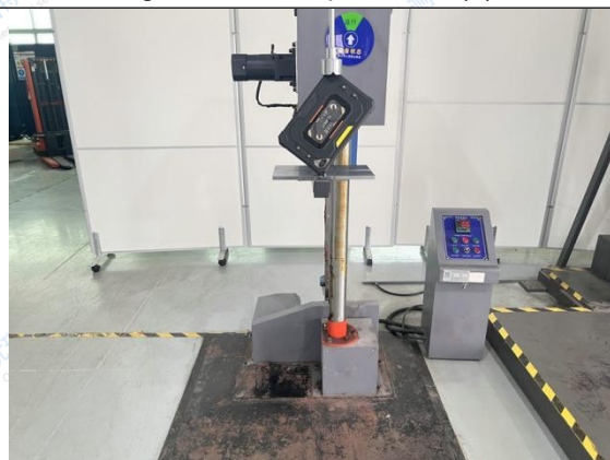
Fig.67 Test setup- Corner (8)
